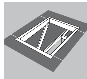
Opening ends short of the rafter, install jack rafter
